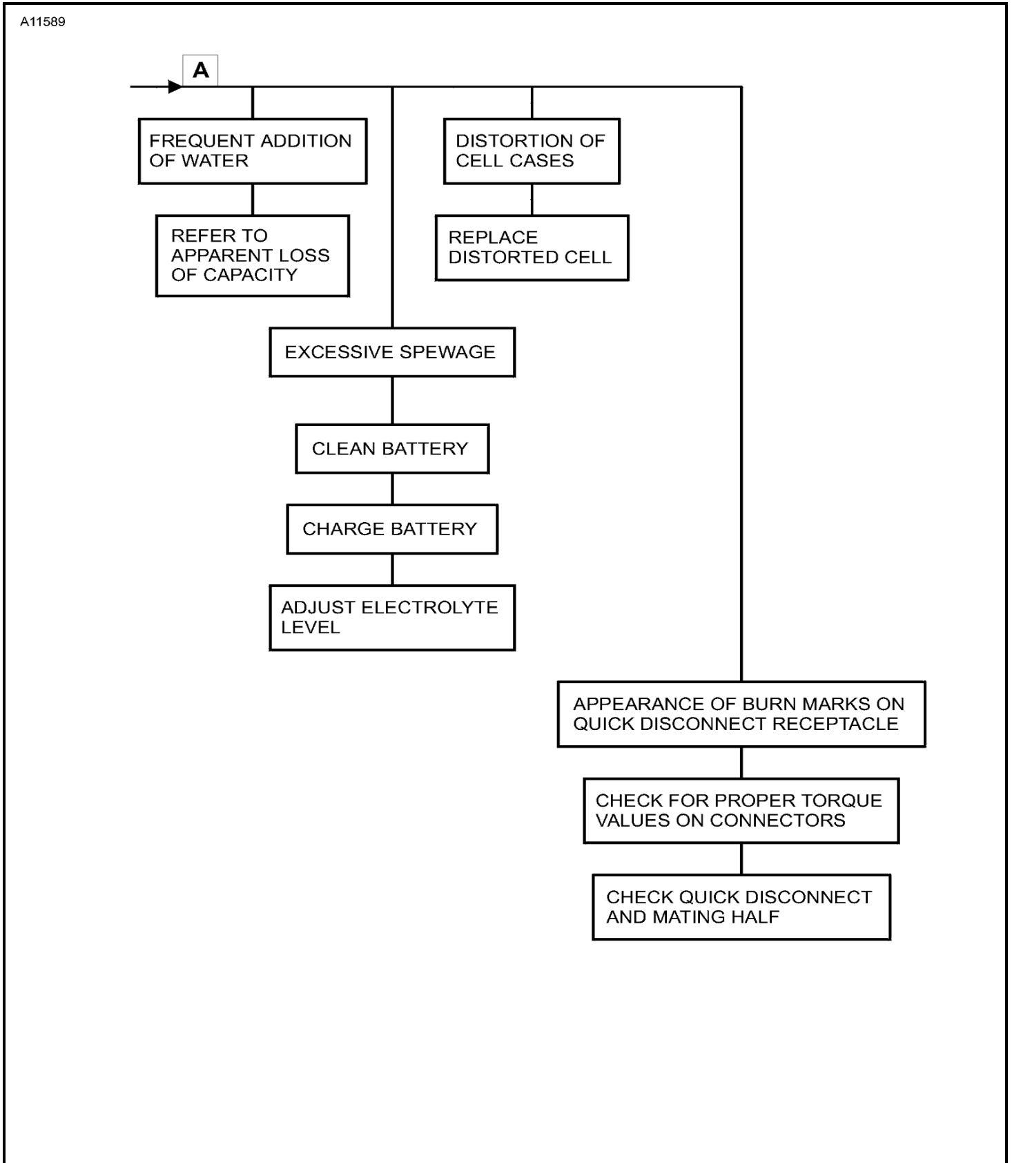
Figure 101 : Sheet 2 : Ni-Cad Battery Troubleshooting Chart
