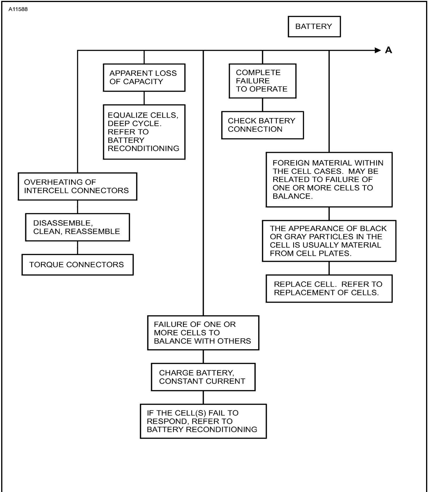
Figure 101 : Sheet 1 : Ni-Cad Battery Troubleshooting Chart
